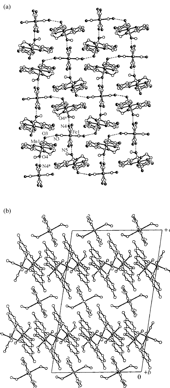
Fig. 2 (a) Hydrogen-bonded two-dimensional network structure for 1 , in which a net unit is consisted of a hydrogen bonded cyclic [⋯(MeOH)Mn(H 2 O)⋯NC–Fe–CN⋯] 4 . (b) Perpendicular view against the projection of 2-D network, [K(18-crown-6)(MeOH)] 2 + cations are located in the interlayers arranged in a one-dimensional column.
