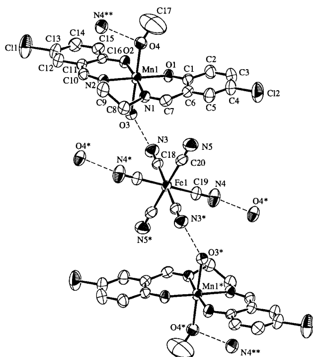
Fig. 1 ORTEP drawing of the [Mn 2 Fe] unit for 1 composed of hydrogen-bonded trinuclear species, [Mn(5-Clisalen)(H 2 O)(MeOH)] 2 [Fe(CN) 6 ] − with the atom numbering scheme of the unique atoms.
